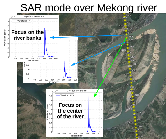
Figure 8. Illustration of SAR waveforms over the Mekong river: the higher resolution provided by SAR mode (300 m along-track) allows to acquire waveforms on illuminated surfaces that are 64 times smaller than LRM ones. As a result, waveforms built from stacks of ground point centered on river beds should often be less affected by land contamination. This assumption is true for this example but might be wrong for others, depending on the river’s orientation relative to the satellite ground track. (Data from ESA/ESRIN EOP/SER prototype.)
